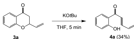
Scheme 3. Base mediated retro-Michael reaction of 3a .
